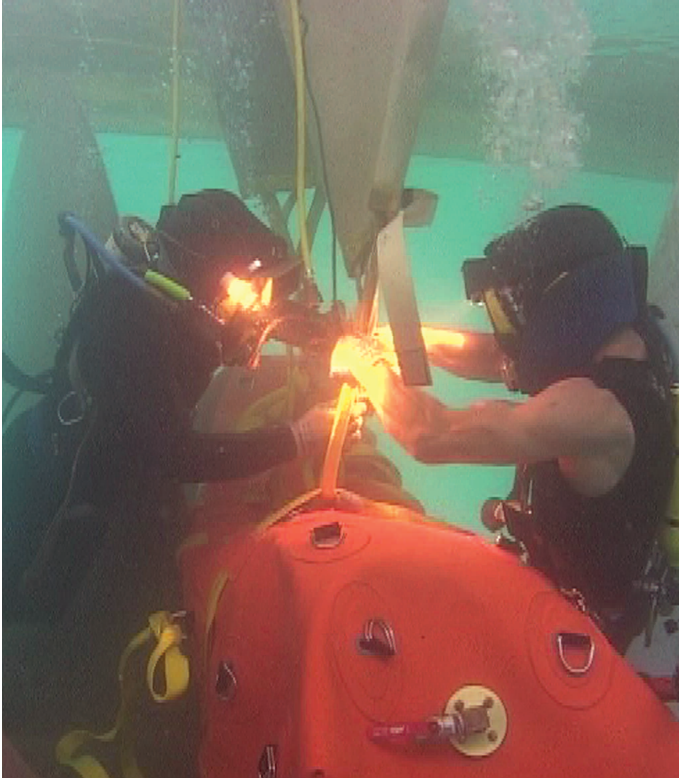
Underwater Stern tube Seal Replacement and Repair
